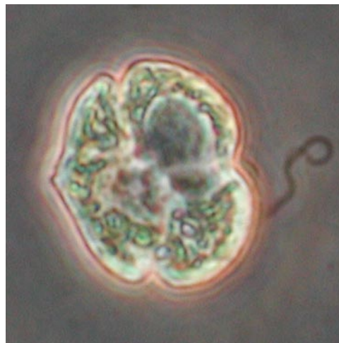
Microscopic view of Karenia brevis cell
